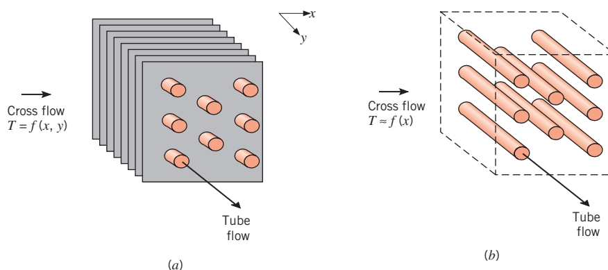
FIGURE 11.2 Cross-flow heat exchangers. (a) Fined with both fluids unmixed. (b) Unfined with one fluid mixed and the other unmixed.
